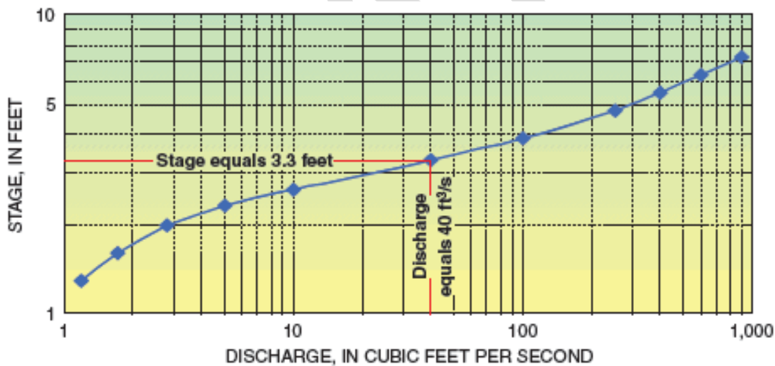
Figure 4-1. Stage-Discharge Rating Curve
