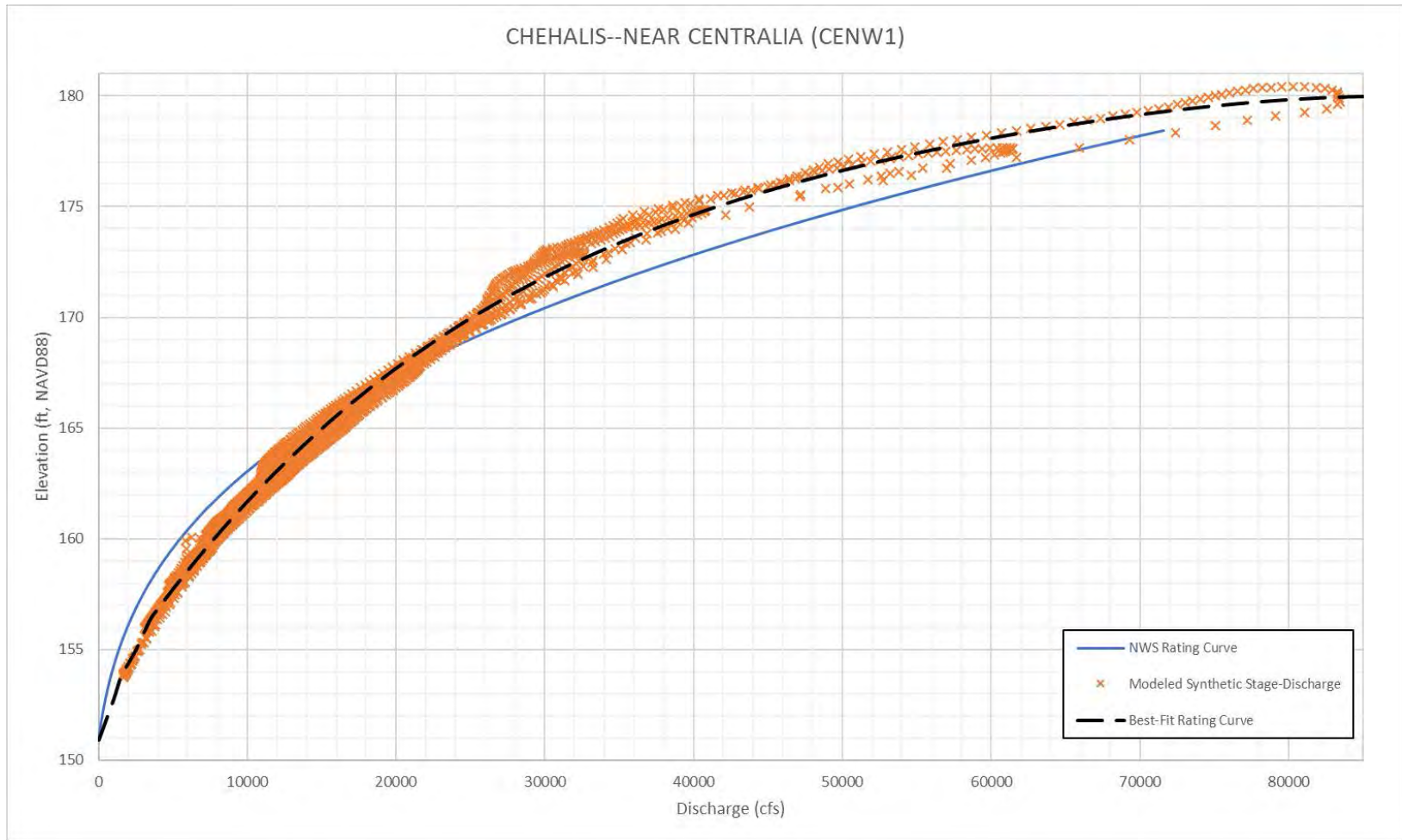
Figure 4-9. Chehalis River near Centralia (CENW1) Rating Curves
