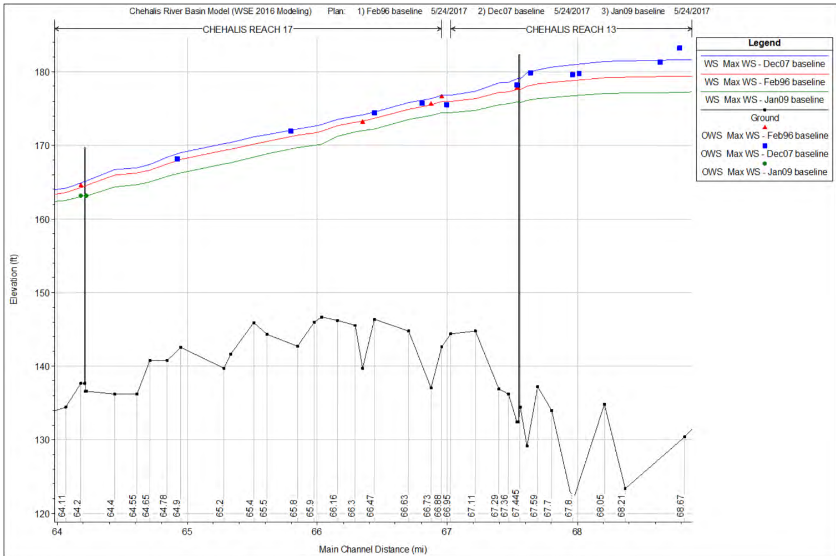
Figure 4-4. Chehalis River Longitudinal Profile
