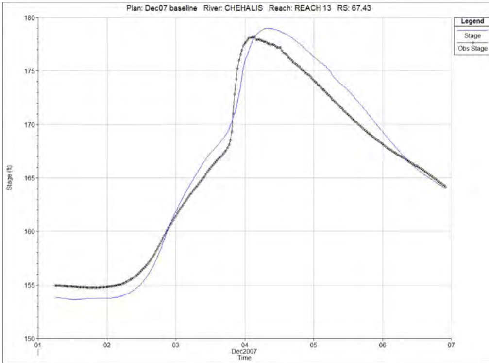
Figure 4-6. Observed vs Simulated Results at CENW1 (December 2007)
