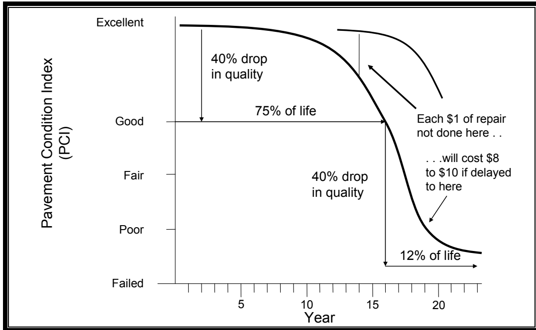
Figure 10. Typical Pavement Deterioration Curve
