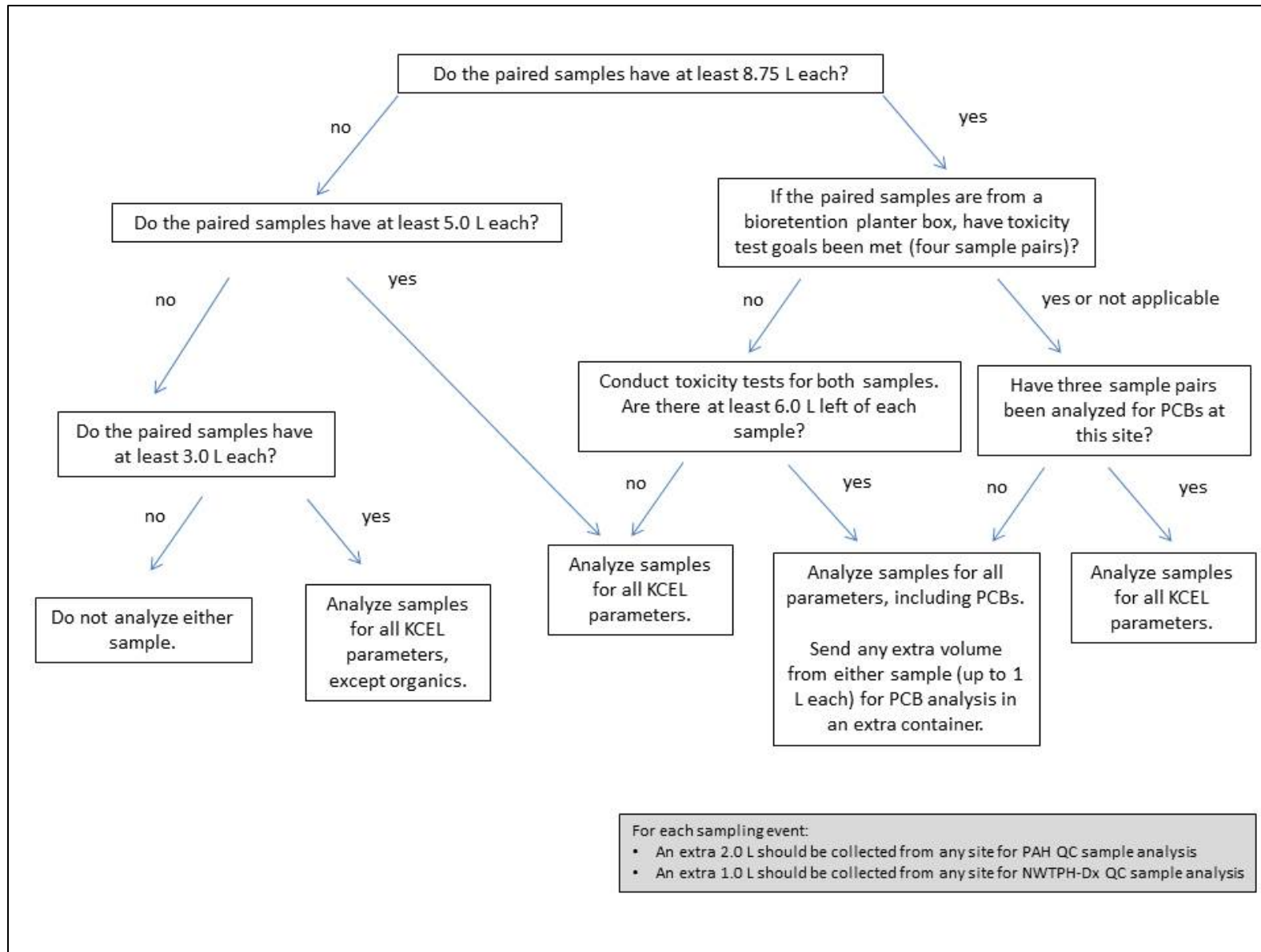
Figure 3. Sample Analysis Decision Tree Based On Paired Sample Volume
