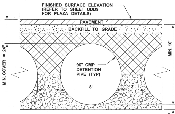
CMP DETENTION SYSTEM - TYPICAL SECTION VIEW N.T.S.
