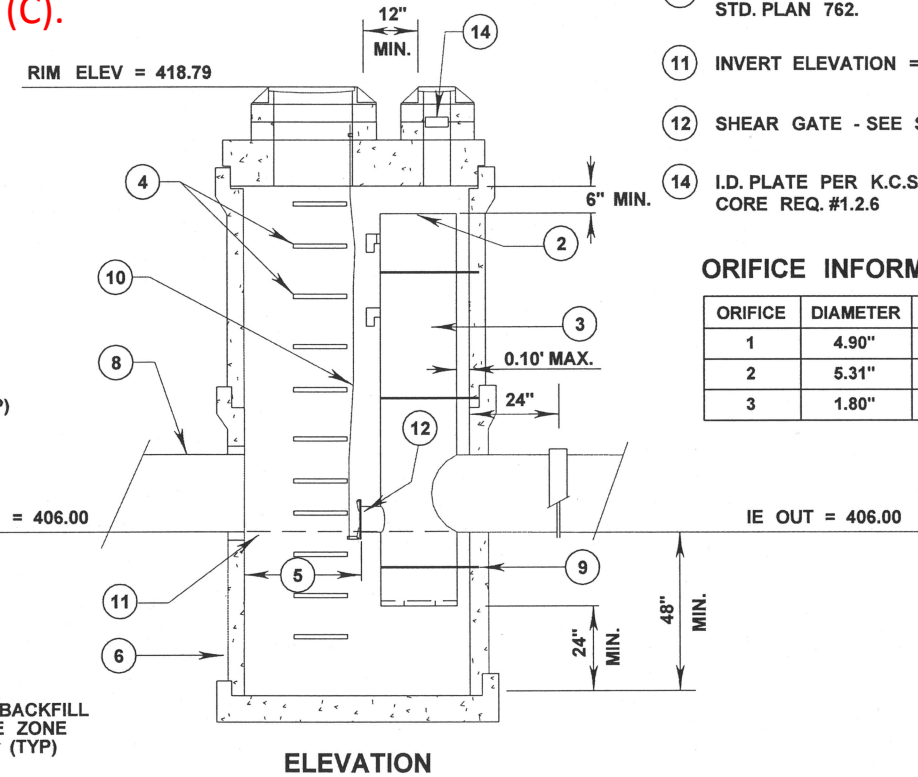
FLOW CONTROL STRUCTURE DETAILS (DR4-31) N.T.S.
