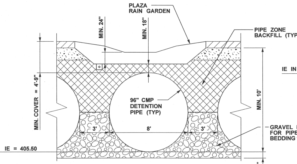
CMP DETENTION SYSTEM - SECTION VIEW AT RAIN GARDEN N.T.S.
